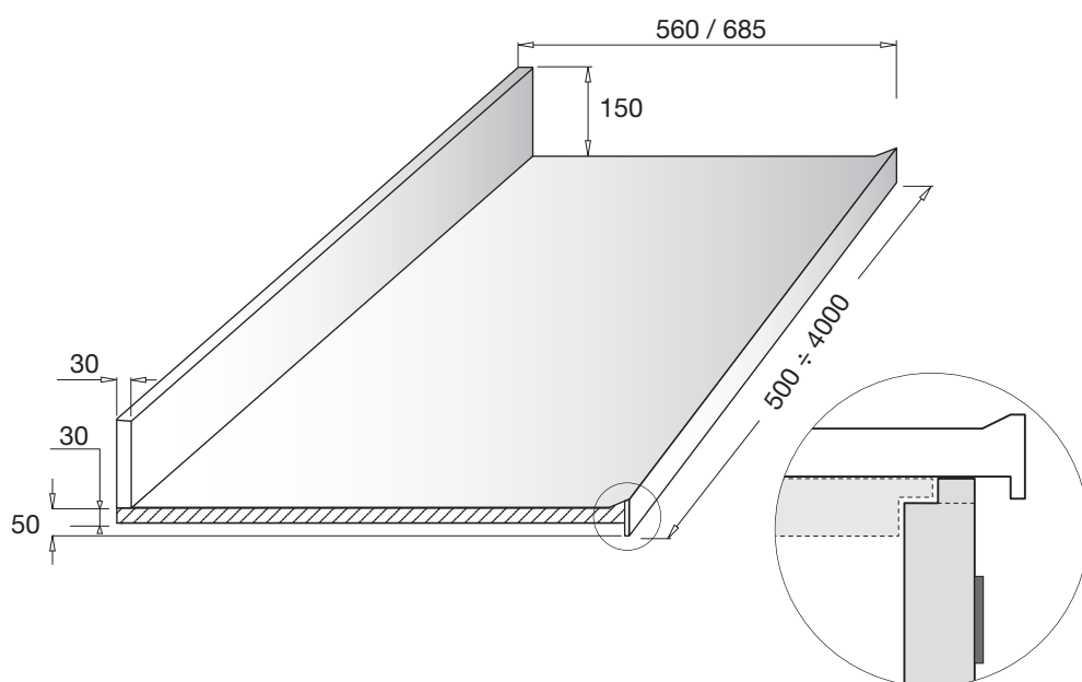
Piano con alzatina posteriore, supporto bancalina e bordino salvagoccia • Top with splashback, support for the top holder and raise border
