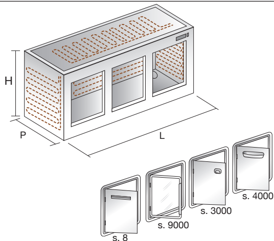
Cella 3 fori • Counter 3 holes
