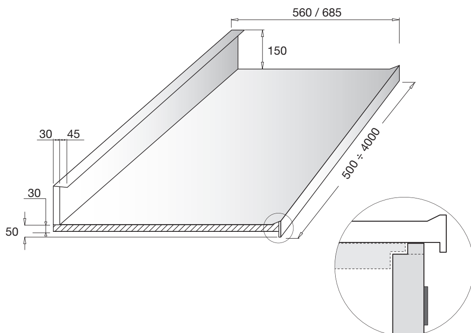
Piano con alzatina posteriore, supporto bancalina e bordino salvagoccia • Top with splashback, support for the top holder and raise border
